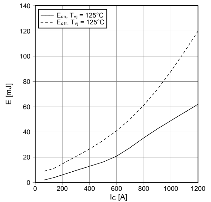
Schaltverluste IGBT-Wechselr. (typisch) switching losses IGBT-inverter (typical) E_{on} = f(I_C) , E_{off} = f(I_C) V_{GE} = \pm 15\text{ V} , R_{Gon} = 0.5\ \Omega , R_{Goff} = 0.5\ \Omega , V_{CE} = 600\text{ V}
